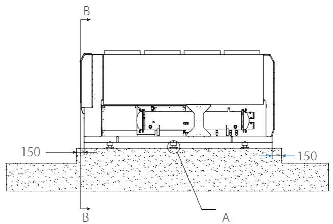
Layout A
